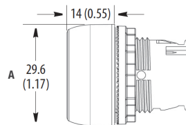
Spring Return Shrouded Push Button
